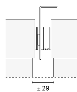
Intermediate bracket
